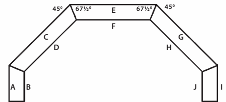
45 DEGREE OUTSIDE CORNER WITH 90 DEGREE ENDS
