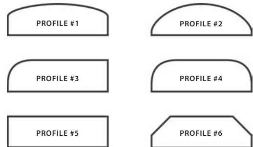
SIDE VIEW OF RAIL
