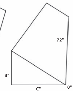
Wedge #14
