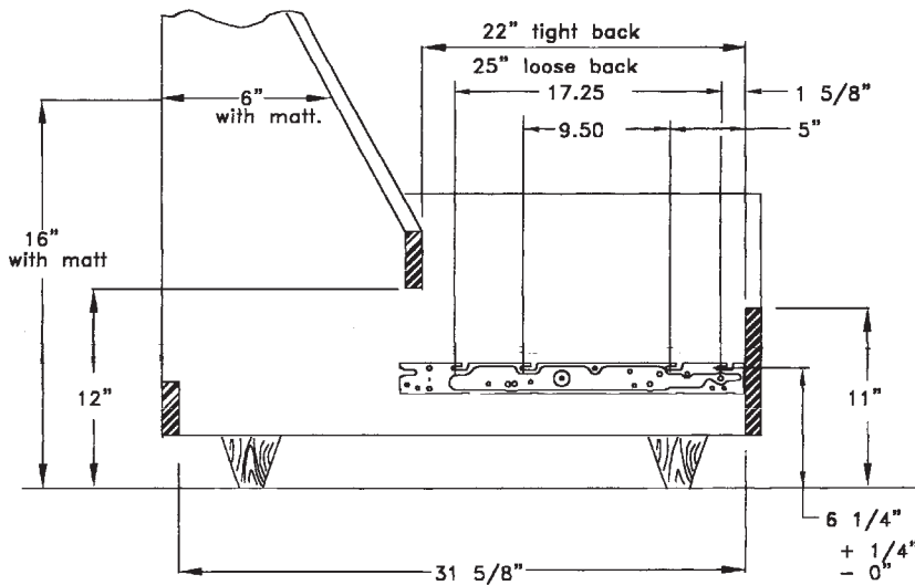
Contoured seat section
