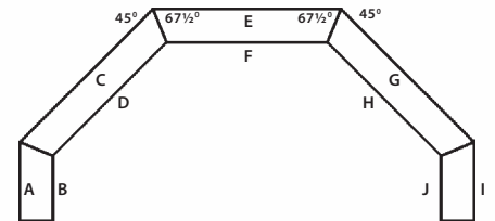
45 DEGREE OUTSIDE CORNER WITH 90 DEGREE ENDS
