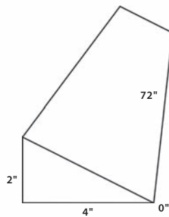
Wedge #11
